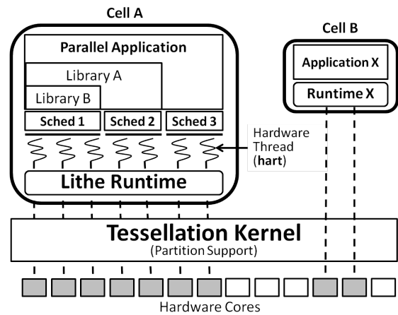
Figure 5. Hierarchical composition of parallel libraries via Lithe within a Tessellation’s Cell.
