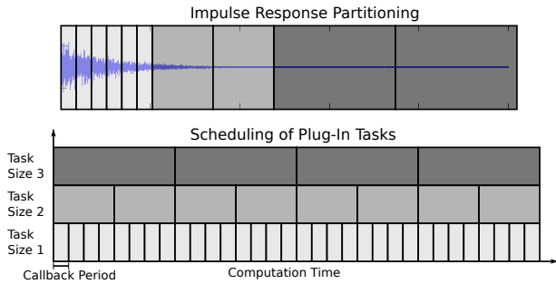
Figure 2. Top - Partitioning scheme for an impulse response using increasing block sizes. Bottom - Scheduling requirements for the tasks for each block size.
